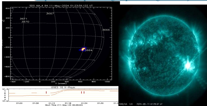
Figure 2: The X5.8 solar flare of May 11, 2024 at 01:23 UT peak time (from https://www.lmsal.com/solarsoftandhttp://sdo.gsfc.nasa.gov/data/aiahmi/ ).
